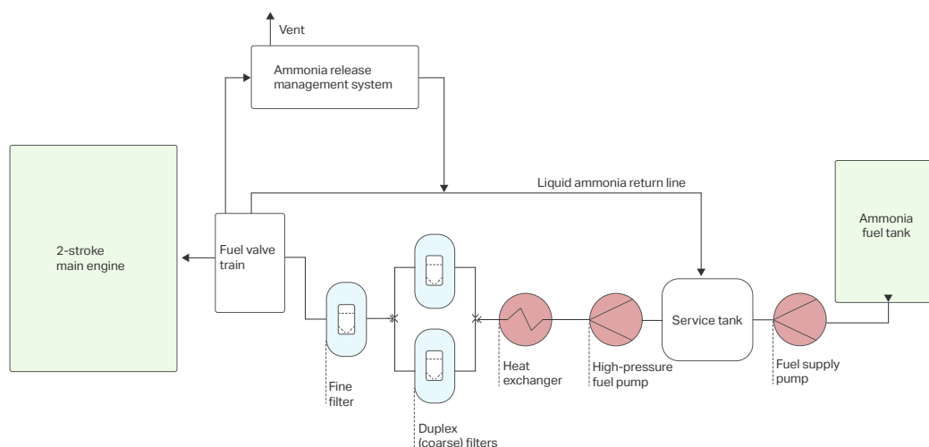
Figure 11: An example of a high-pressure ammonia fuel supply system.
